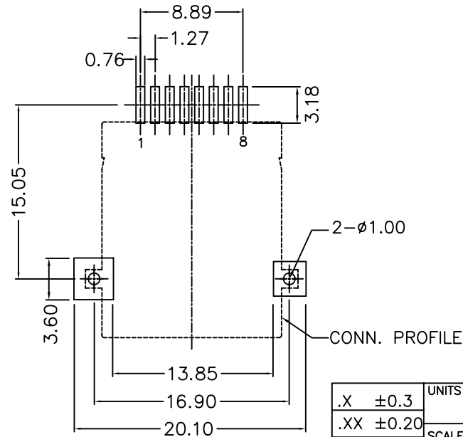
PCB LAYOUT
