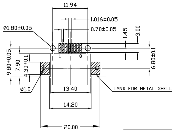
PCB LAYOUT
